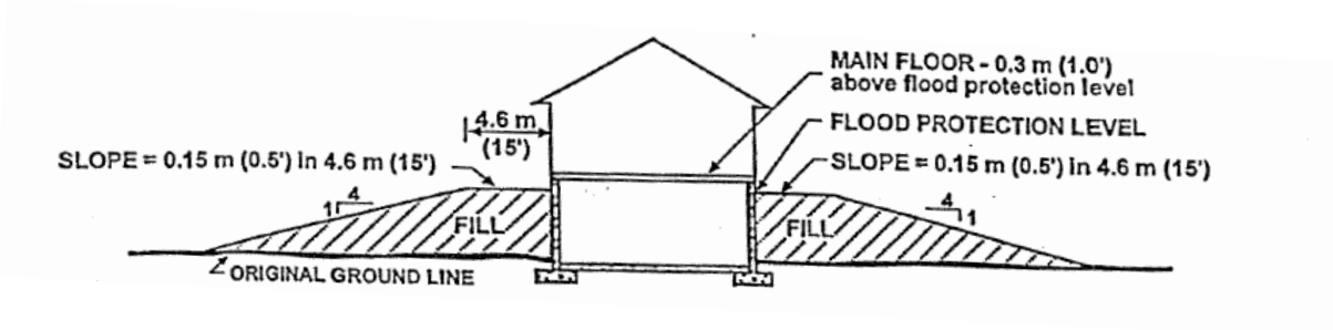
Schedule B – Structure with no basement or cellar
