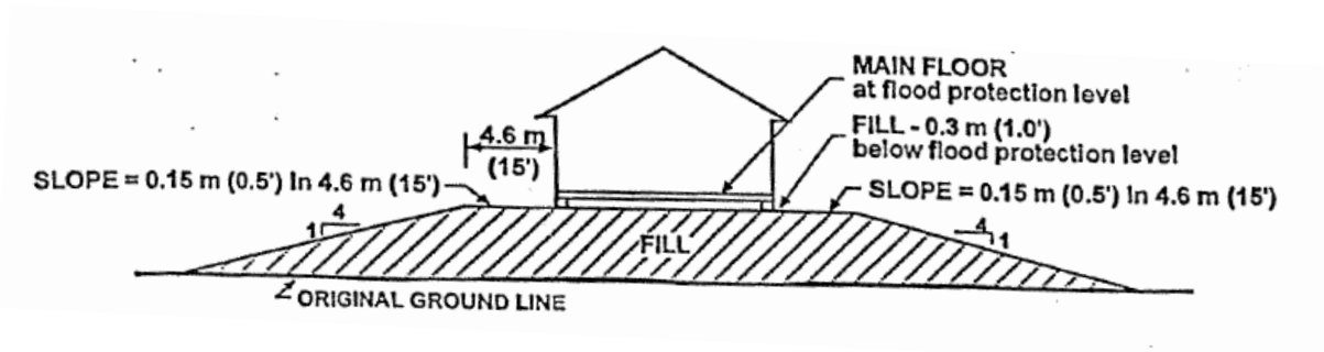
Schedule C – Elevated structure
