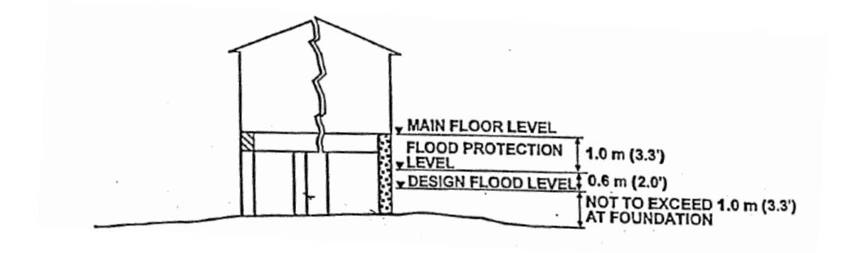
Schedule C – Elevated structure
