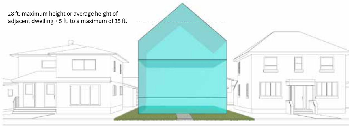
Building height guidelines
