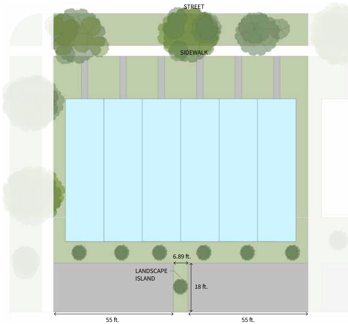
This image demonstrates the landscaping requirements within the parking area of a multi unit residential dwelling.
